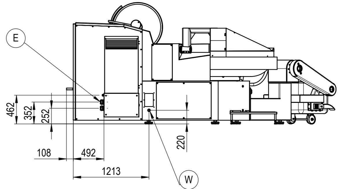
ANSICHT "A" / VIEW "A"
